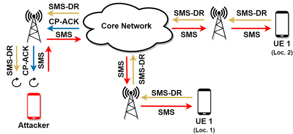
Figure 3: Network flow for SMS transmissions in different locations.
